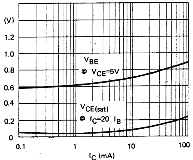
V BE AND V CE(sat) vs COLLECTOR CURRENT
