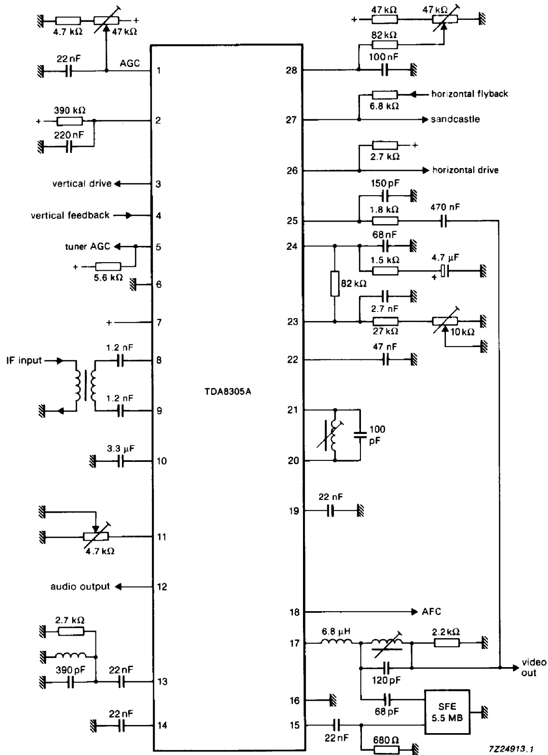
Fig.11 Application diagram.
