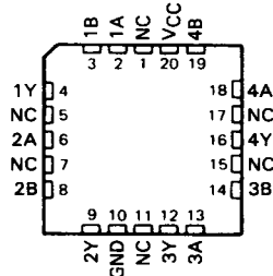
SN54HC08 . . . FK PACKAGE (TOP VIEW)
