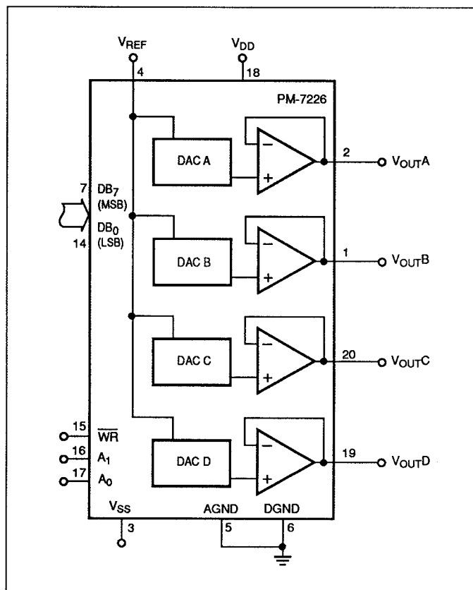
FIGURE 15: Unipolar Operation
