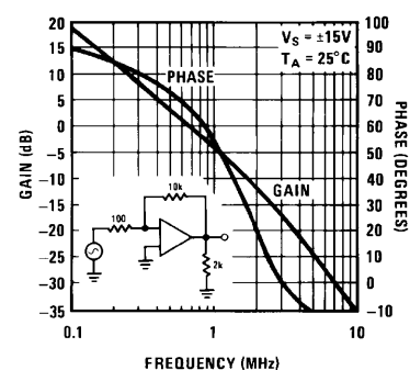
Bode Plot LM148
