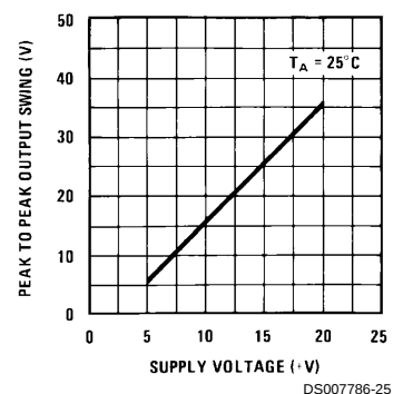
Voltage Swing
