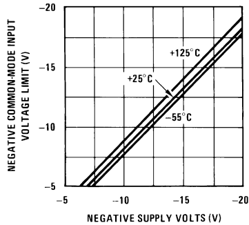
Negative Common-Mode Input Voltage Limit
