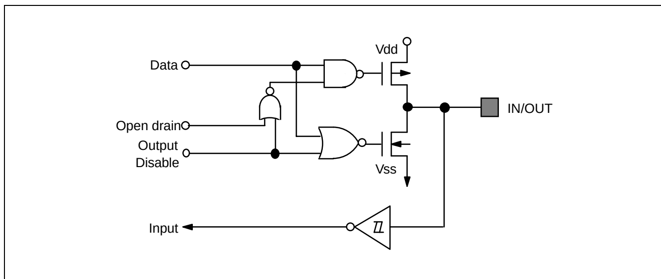
Figure 1-8. Pin Circuit Type E-1
