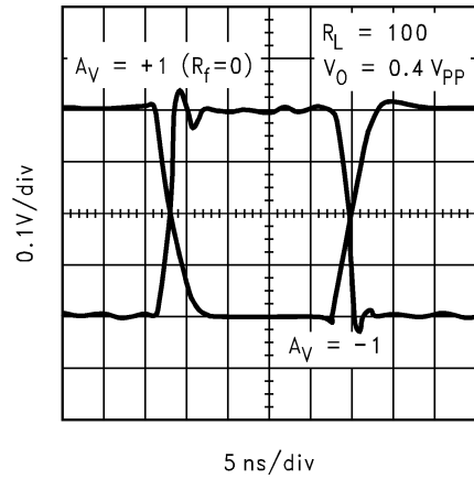
Pulse Response
