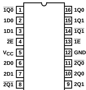
CD54HC75, CD54HCT75 (CERDIP) CD74HC75 (PDIP, SOIC, SOP, TSSOP) CD74HCT75 (PDIP, SOIC) TOP VIEW
