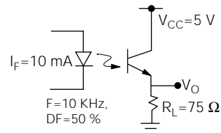
Figure 2. Non-saturated switching timing
